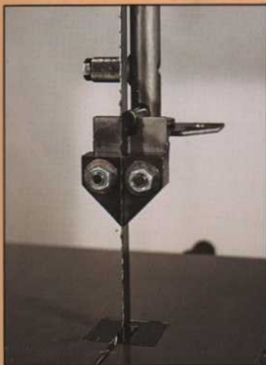
Upper and lower guide unit has simple blocks with large working faces. Adjustable for blades up to 16 mm ( \frac{5}{8} in) wide. (Shown with guard removed.)
